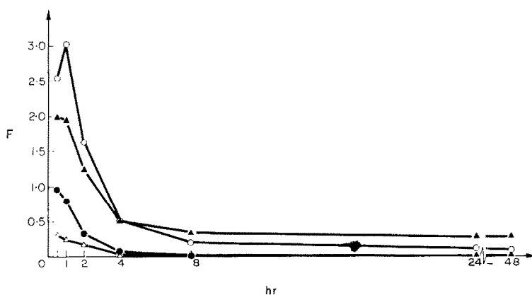
FIG. 1. Distribution of ^{14}C -psilocin in the kidneys ○—○, liver ▲—▲, brain ●—●, blood △—△.
